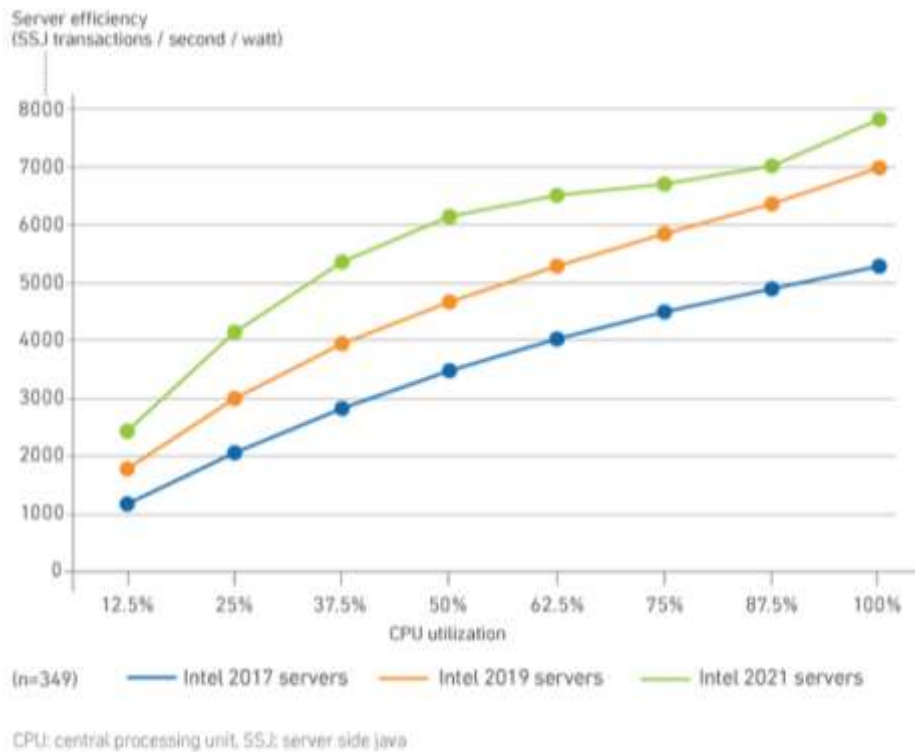
Figure 3.3 Efficiency improves with each Intel server generation 4
